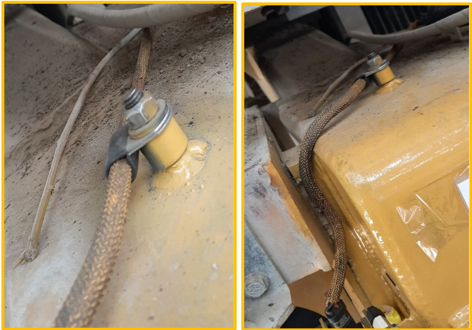
Harness Fixing Process Before/After - Source: SOTREQ S/A
