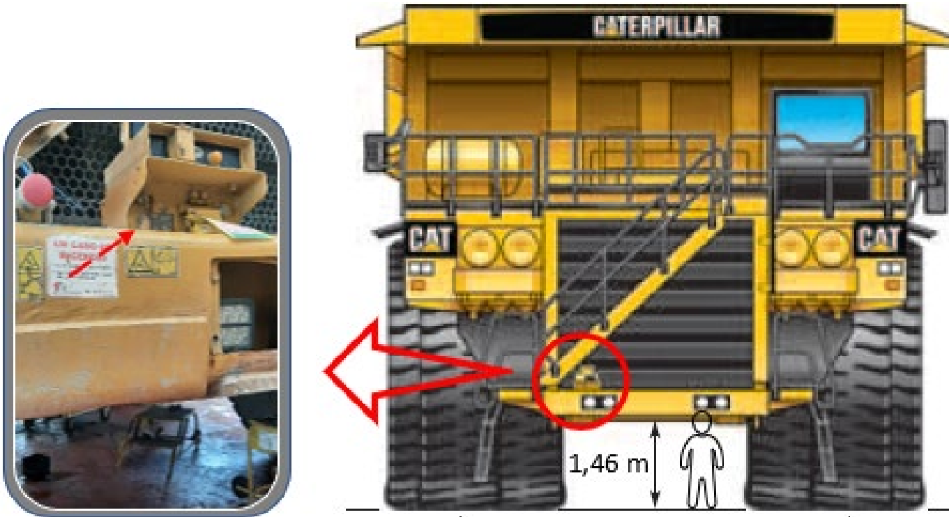
Original position of the Shutdown Switch – Source: SOTREQ/Giesi Nascimento.
